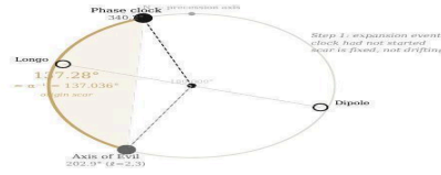
Figure 8: The \alpha -Lag: Origin Scar in the Bilateral Frame
