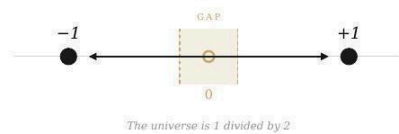
Figure 2: The Seed Condition: \{1, 0, -1\}
