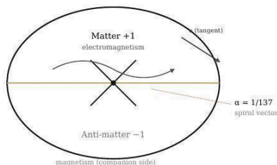
Figure 7: The Cosmic Egg; Matter, Anti-matter, and the Spiral Vector 1/137
